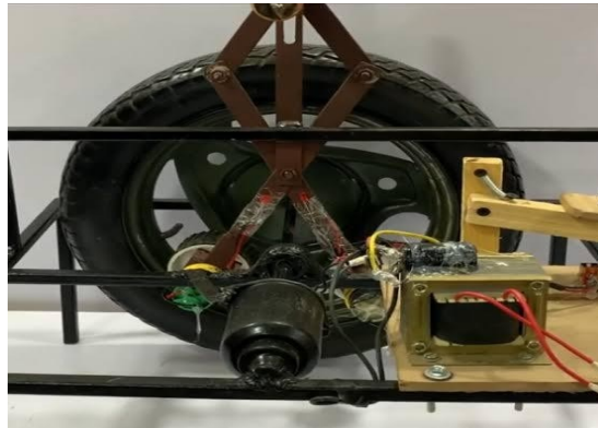
Figure 1:- Regenerative Braking System
